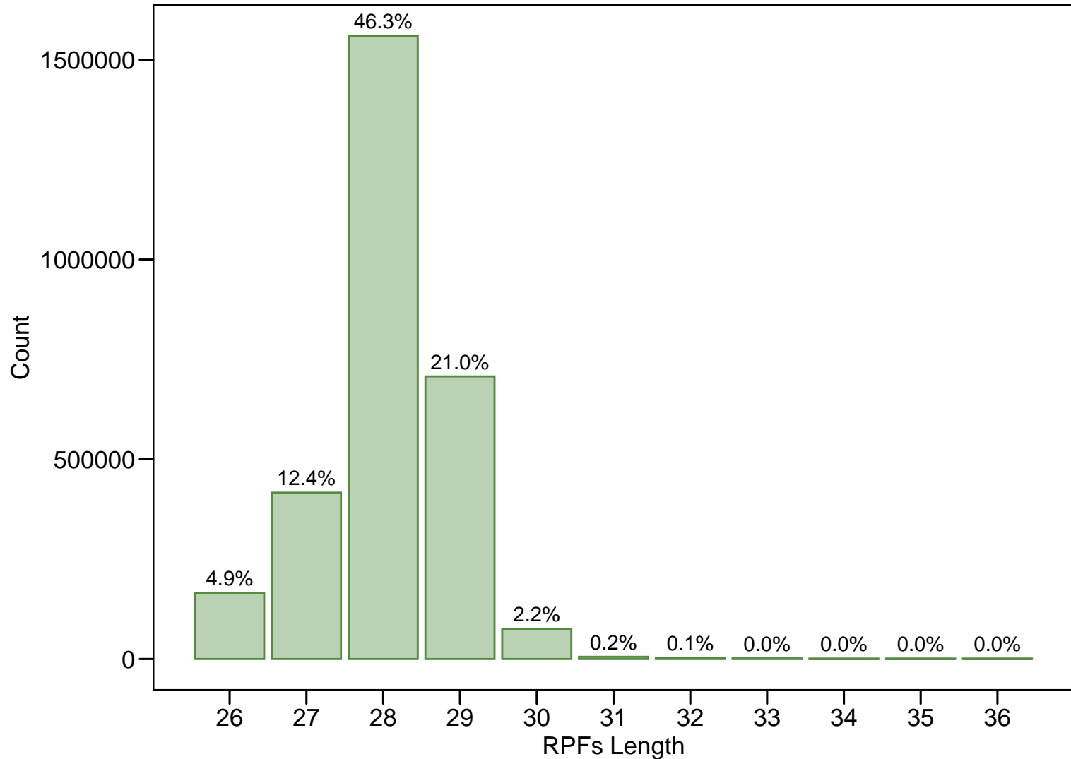
wt_2 Sequence Length Distribution (26–36)
